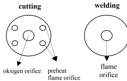
Gambar 2. Tipe torch
