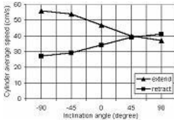
Fig.5. Effect of inclination angle to cylinder average speed with load of 5 kg
