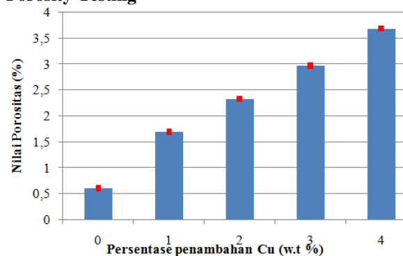
Figure 2 Porosity testing result graph
